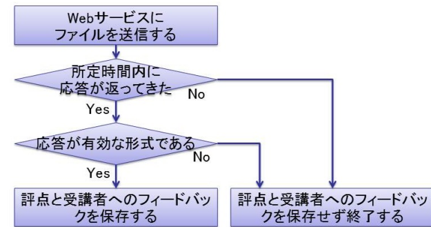
図 6 提出時の応答確認 Fig. 6 Flow of Checking Response on Submission
