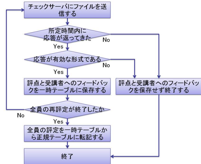
図 7 再評価時の応答確認 Fig. 7 Flow of Checking Response on Regrading
